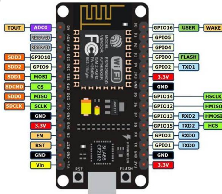
Figure 3: NodeMCU pinout
