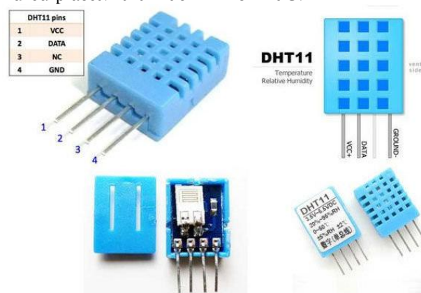
Figure 1: DHT-11 Sensor
