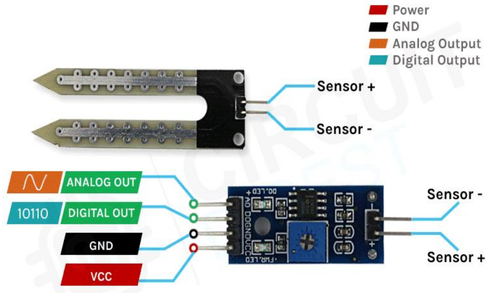
Figure 2: Moisture sensor
