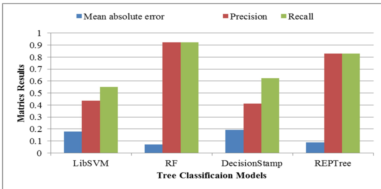
Figure 5. Performance metrics of LibSVM, Random Forest, Decision Stump, and REP Tree classifiers
