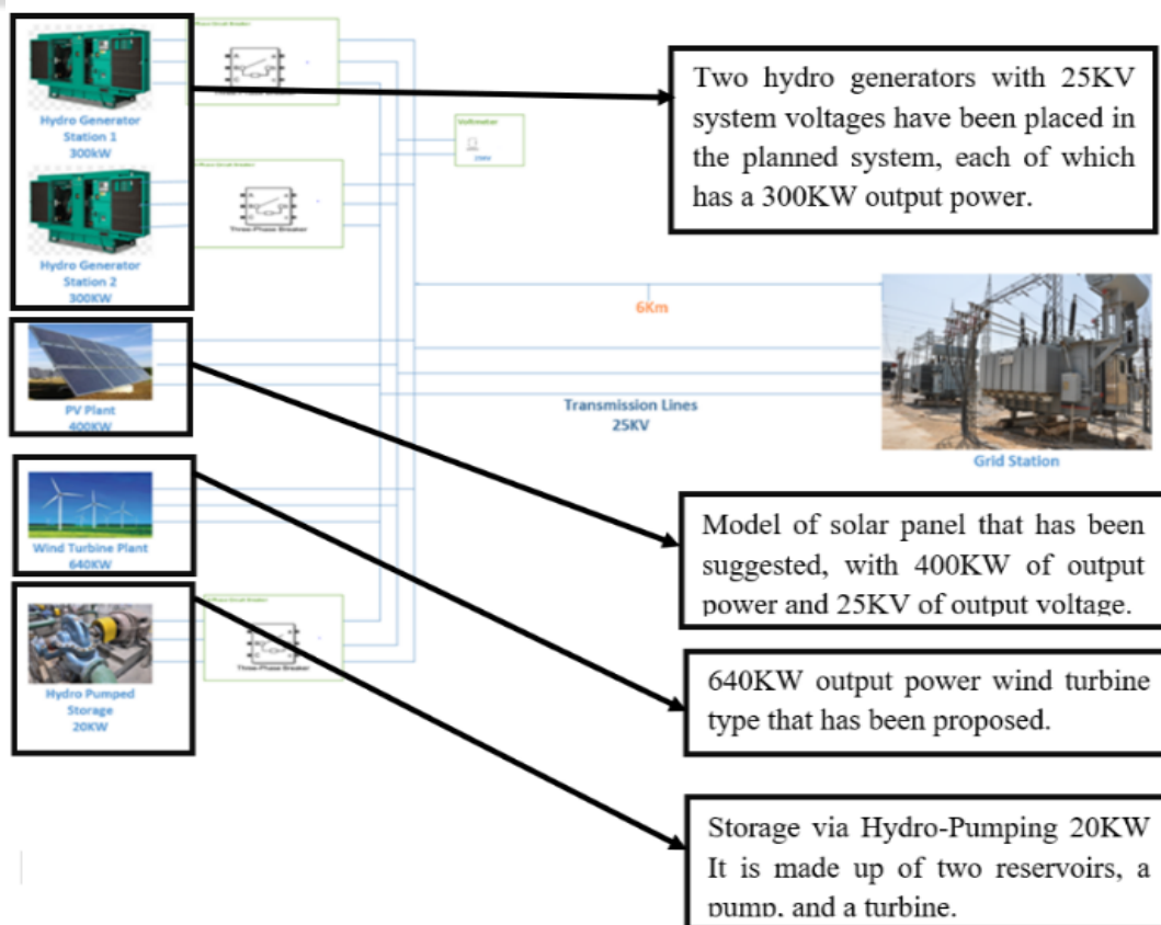
Figure: 4.1 The attached Visio model, which has 25 KV transmission lines connected to a grid station, offers the most lucid conclusion and justification for our effort.
