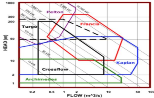
Figure 5.3. Chart depicts the working ranges of each turbine in terms of head and stream rate.
