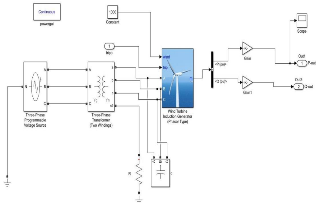
Fig. 3.2. 640KW output power of proposed wind turbine model (Simulink).
