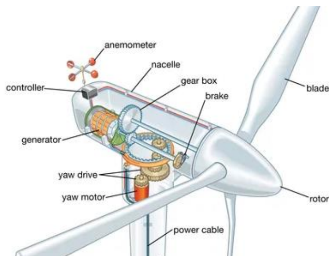
Figure 2.2. Wind turbine diagrammatic example [31].
