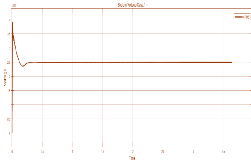
Figure 4.3.1. Showing the system's 25 KV output voltage indicates system stability and the usage of extra produced electricity for water pumping.
