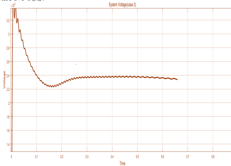
Figure 4.3.3. Demonstration of how the system voltage lowers from 25 KV to 24 KV when the connected load exceeds the power generated.
