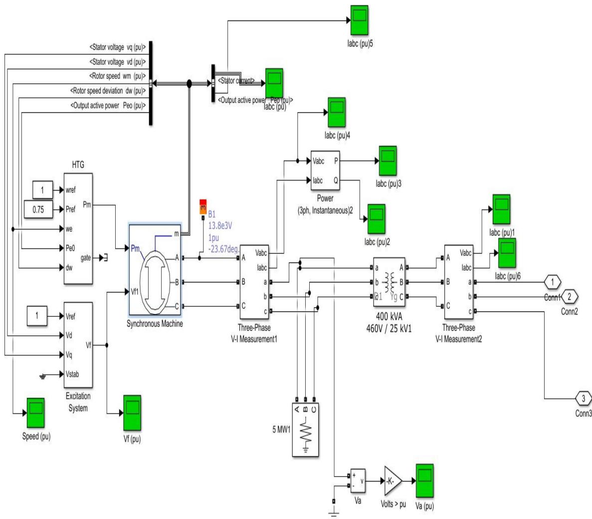
Fig.3.4: Simulink model of a 300KW hydro generator; two hydro generators with 25KV system voltages are installed in the suggested system..
