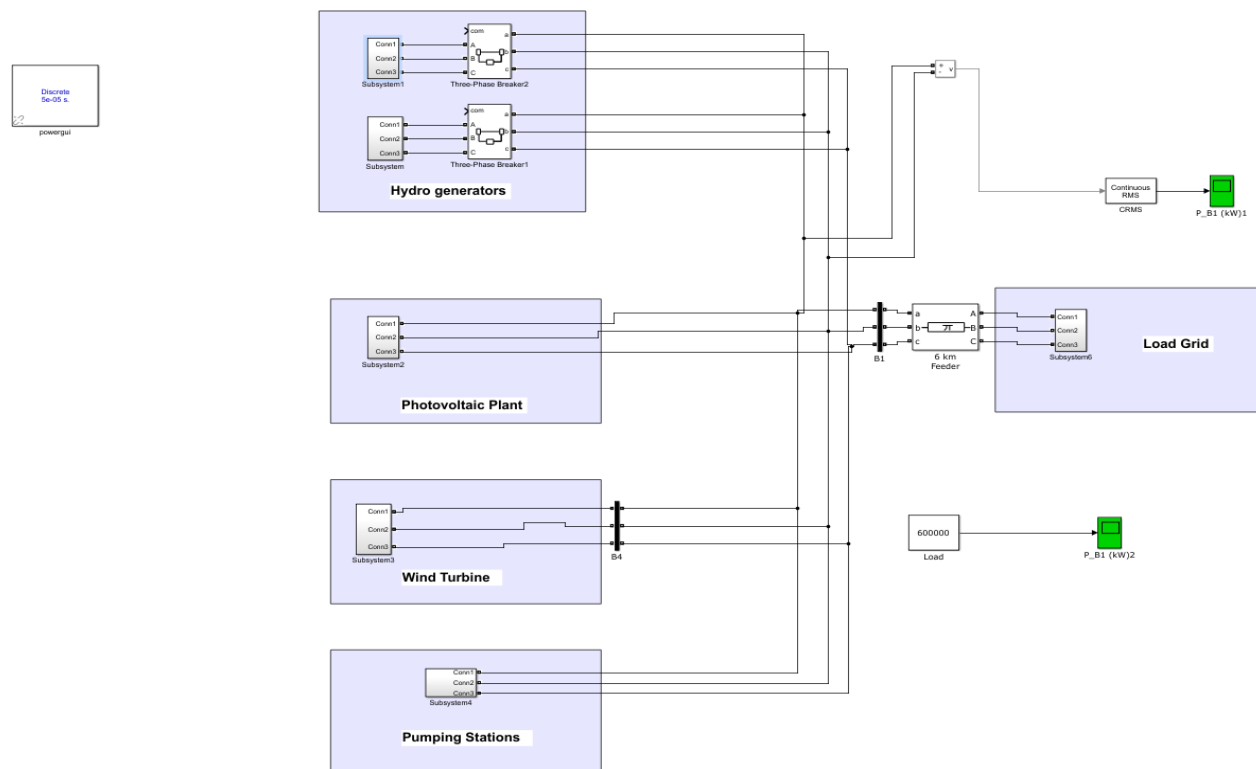
Figure. 4.2: Simulink Prototypes Incorporation
