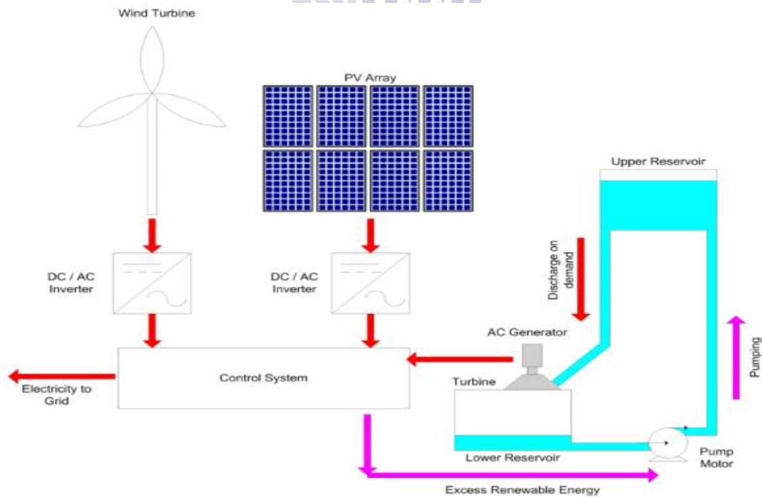
Figure 4.5 In order to integrate and integrate renewable energy sources and meet the growing need for grid station load, pumped hydro storage is being deployed in creative ways.
