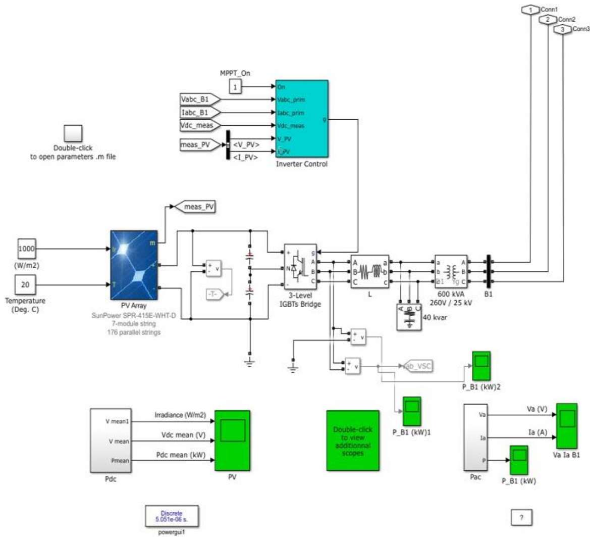
Fig. 3.1. Proposed model of PV with MPPT Controller, Output power 400KW and Output Voltage 25KV (Simulink).
