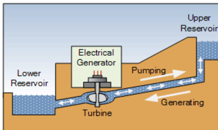
Figure 2.1. Schematic diagram of PHS
