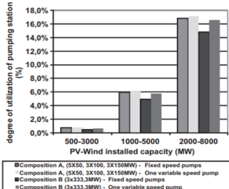
Fig 1.2b The rate of extra wind energy used for pumping, the total amount of pumping station utilization within the two pumping station composition scenarios, the three wind-PV integration scenarios, and the two scenarios with fixed speed pumps or one variable speed pump (up to 12 times).
