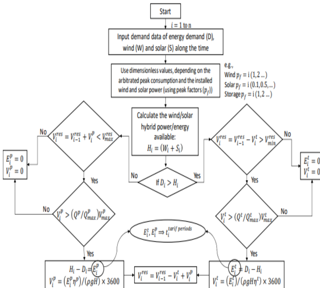
Figure 1.1. Use a flowchart to determine which half-breed system is ideal. The letters V, E, D, and S represent water volume (V), imperativeness (E), request (D), half-breed power/energy (H), sun-oriented essentialness (S), wind essentialness (W), and so on. The superscripts p, t, and rest represent a pump, turbine, and supply, respectively.
