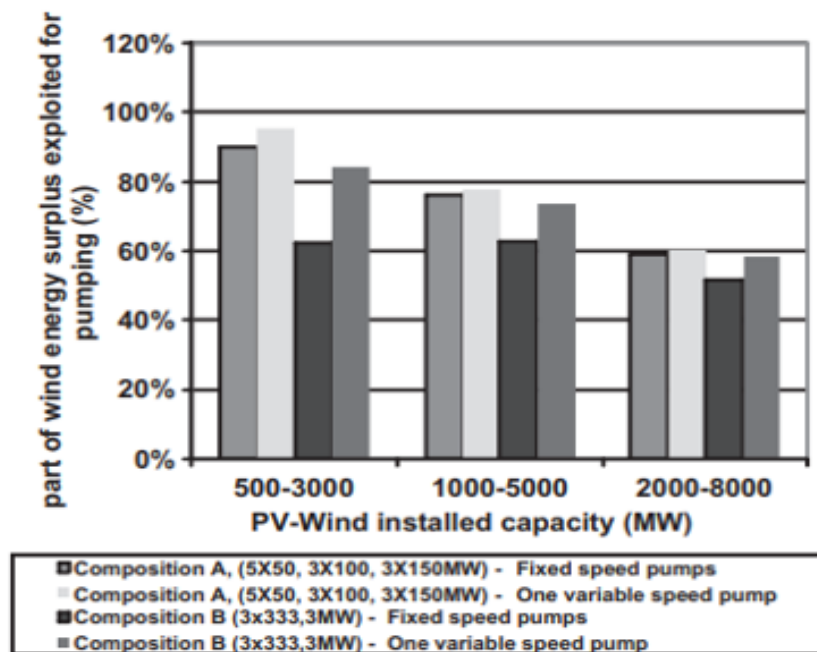
Fig 1.2a The rate of additional wind energy used for pumping, the total amount of pumping station utilization throughout the two pumping station composition scenarios, the three wind-PV integration scenarios, and the two scenarios with fixed speed pumps or one variable speed pump (up to 12 times).
