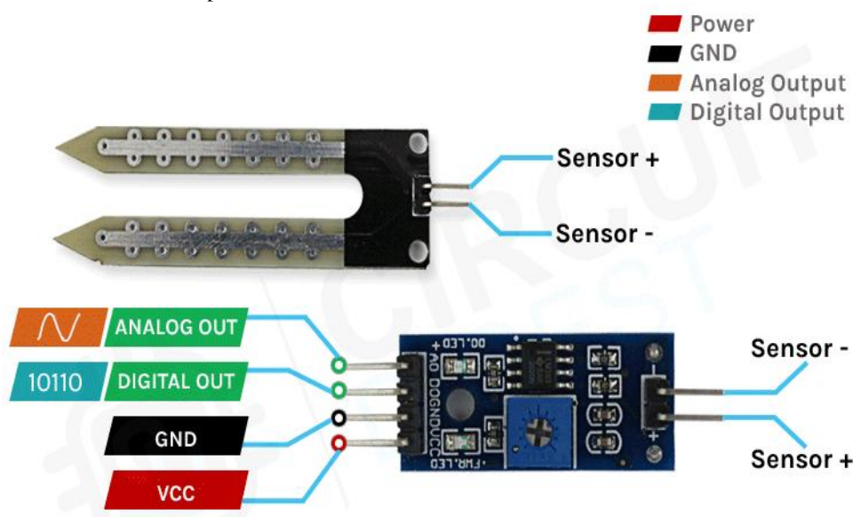
Figure 2: Moisture sensor
