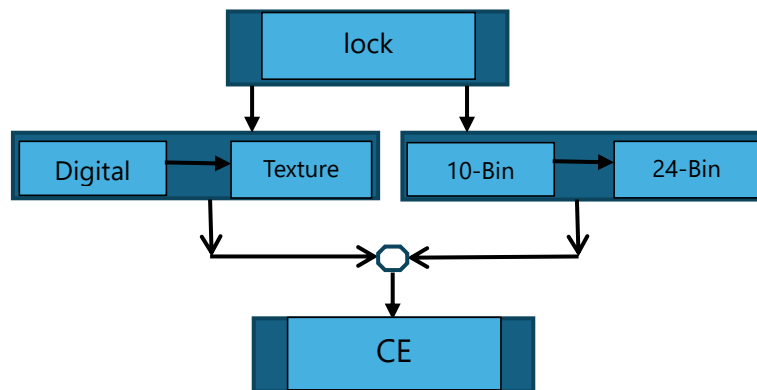
Figure 4 Description of CEDD Feature Detection
