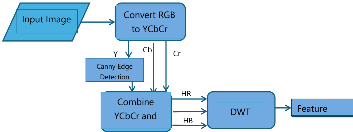
Figure 3 Description of Color-Edge Extraction with Wavelet Transform
