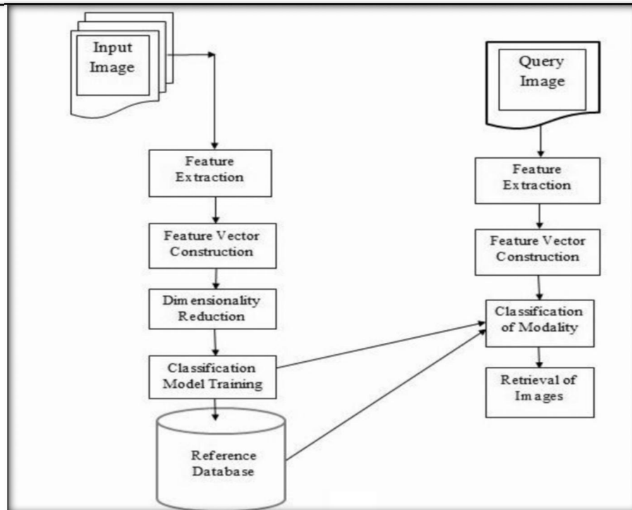
Figure 1 Block Diagram of Proposed Classification Framework
