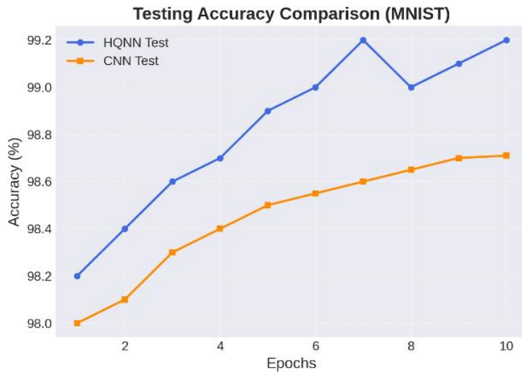
Figure 6 Reported testing-accuracy trend comparison on MNIST.
