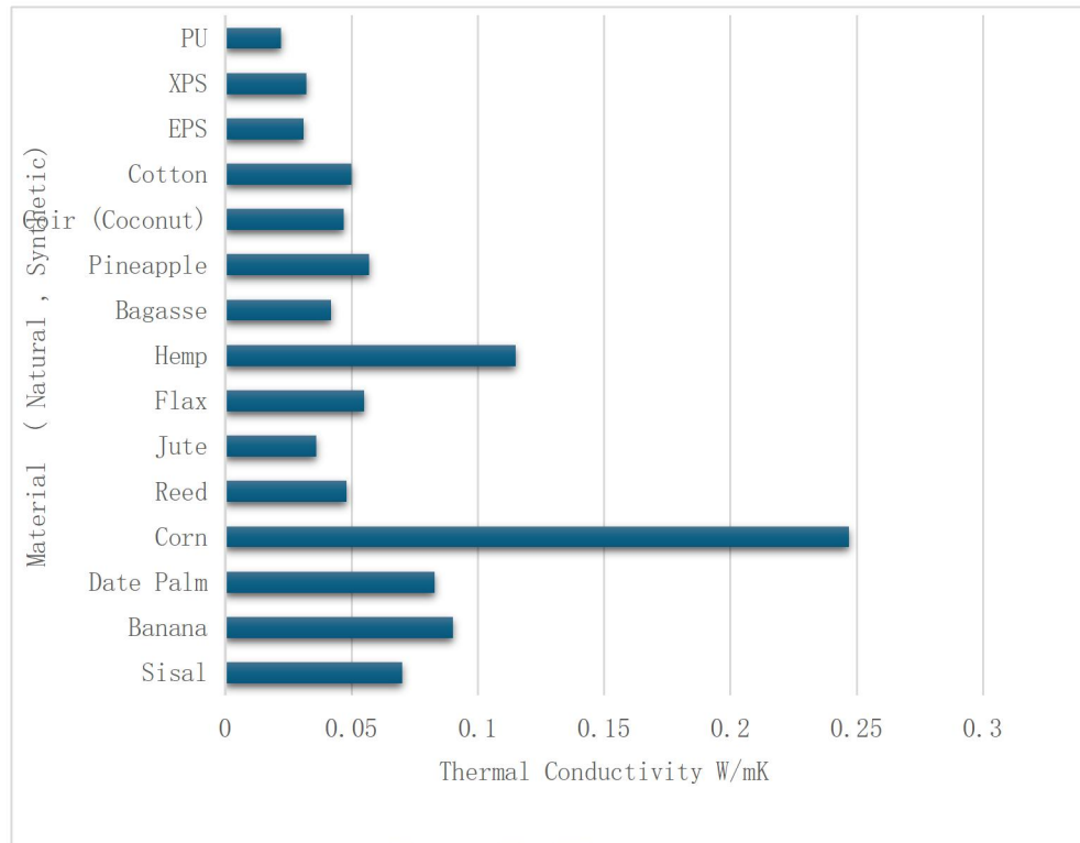
Figure 6: Comparative analysis of Thermal Conductivity of investigated materials
