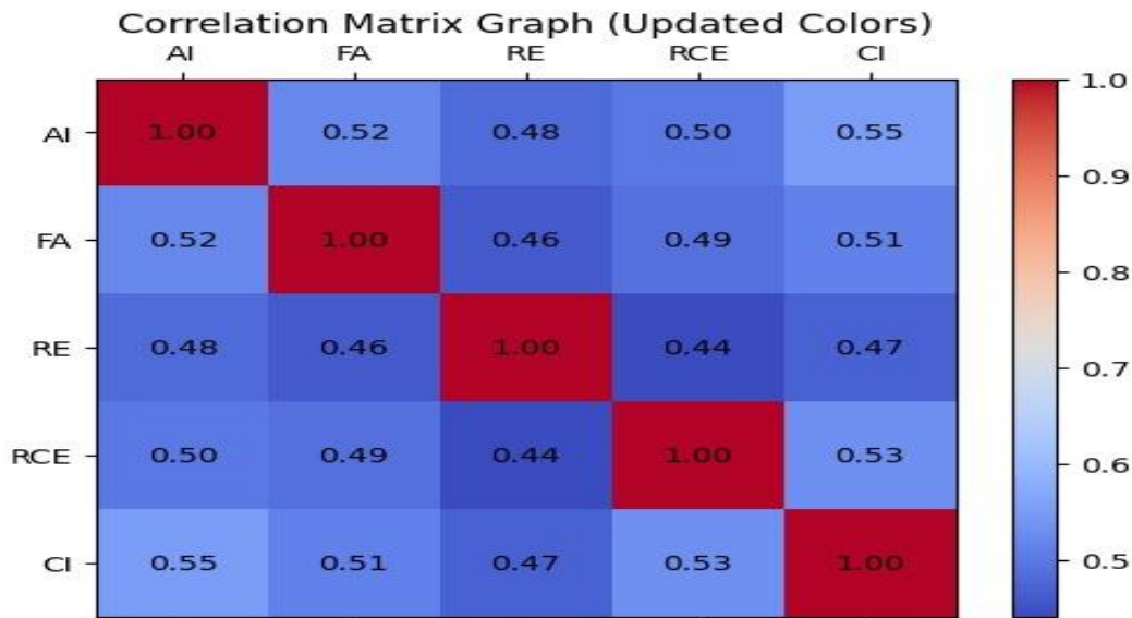
Figure 3. Correlation Matrix
